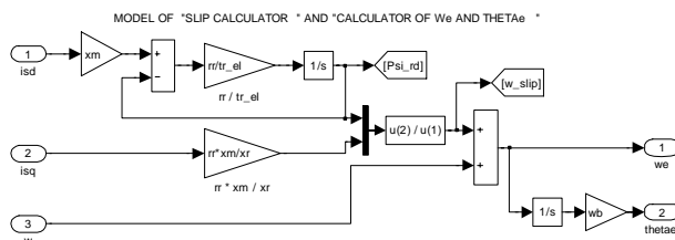
Figure 6 MATLAB/Simulink model of the slip calculator
